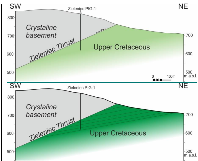
Figure 1718: Schematic section across the Zieleniec Thrust (based on data from Cymerman, 1990, and Kozdrój, 2014). Location in Figs. 2 and 12.
