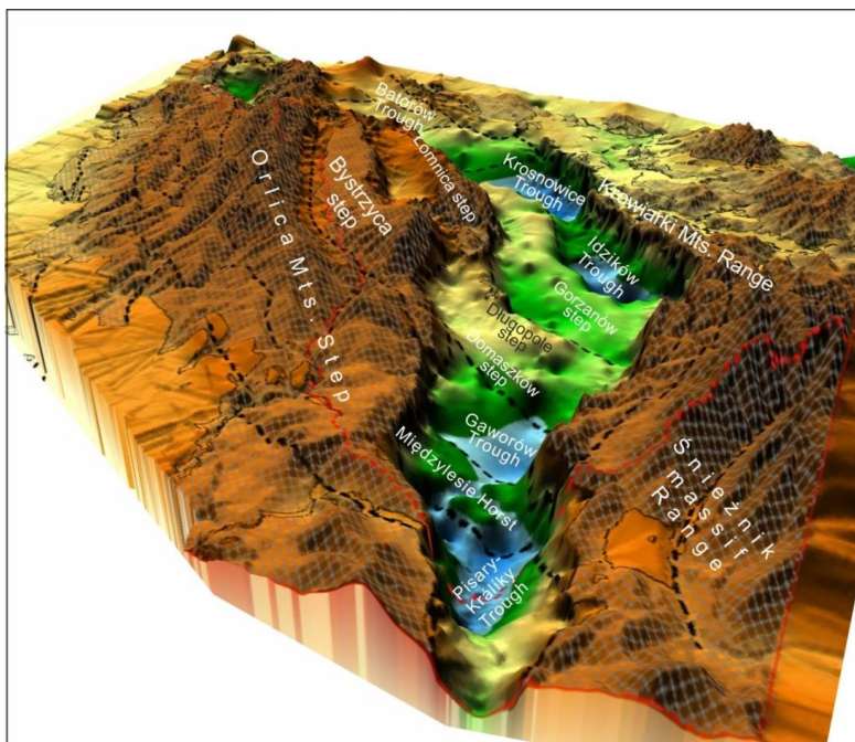
Figure 1617: Perspective view towards the north onto the base Cretaceous relief (known from boreholes) in the Upper Nysa-Králíky Graben (from Badura and Rauch, 2014). The oblique-striking blocks-troughs, steps and horsts reflect NW-SE trending Late-Cretaceous – Early Palaeogene structural grain defined by inverted blocks on underlying the Cretaceous graben floor and folds in its fill (removed from the picture), once continuing laterally, before the graben formed in Miocene times. Location given in Fig. 2.
