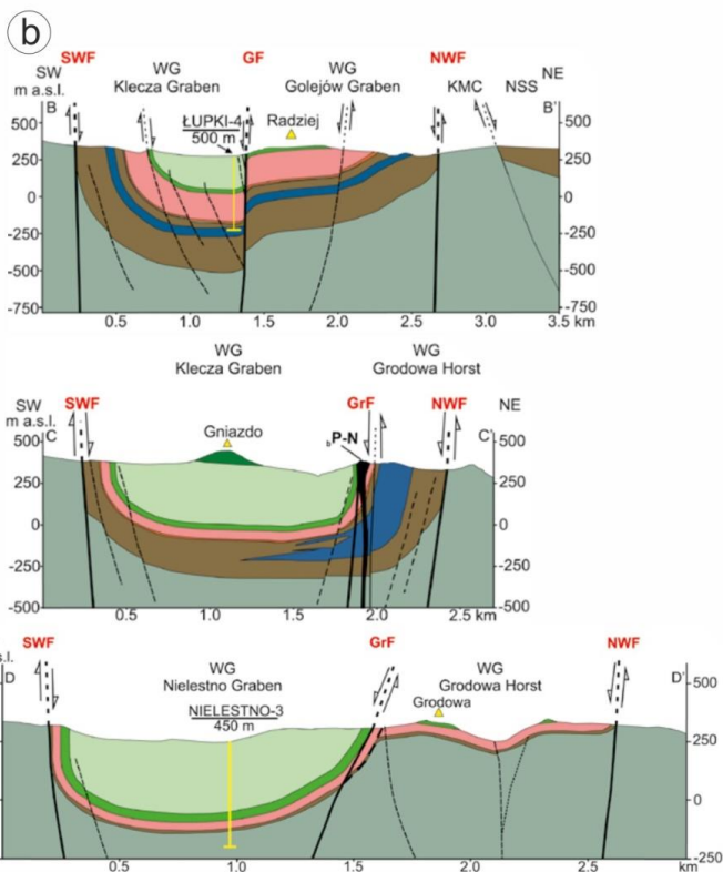
Figure 11: Simplified geological map and three selected cross-sections of the Wleń Graben according to Kowalski (2020)
