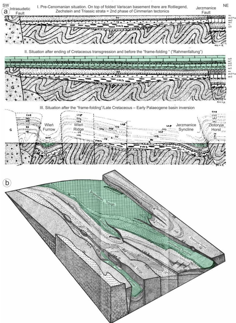
Figure 7: Kurt Beyer's (1939) interpretation of the "young Saxonian" tectonics in the North Sudetic Synclinalorium (Basin).
