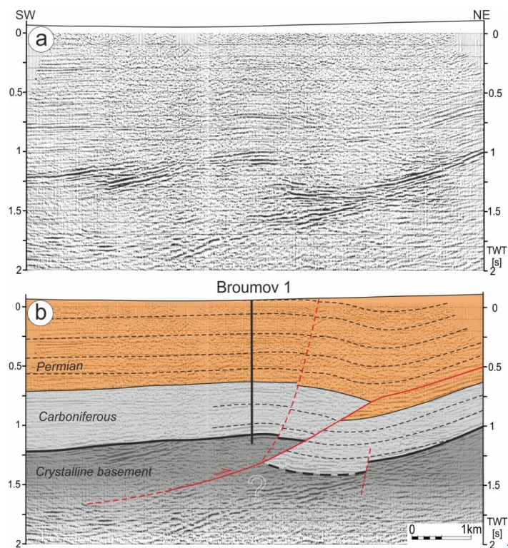
Figure 14 a,b: (a) Seismic profile (paper print version – Brada et al., 1982) from vicinities of Broumov (a) and its interpretation (b) (made on printed paper version – Brada et al., 1982). Location in Fig. 12. The section shows that the Broumov well was drilled in the hanging-wall of a thrust fault and, hence, the Carboniferous in the neighbourhood may occur deeper than found in the well. The thrust continues to the NE parallel to the bedding – most probably along the Permian Anthracosia Shale member.
