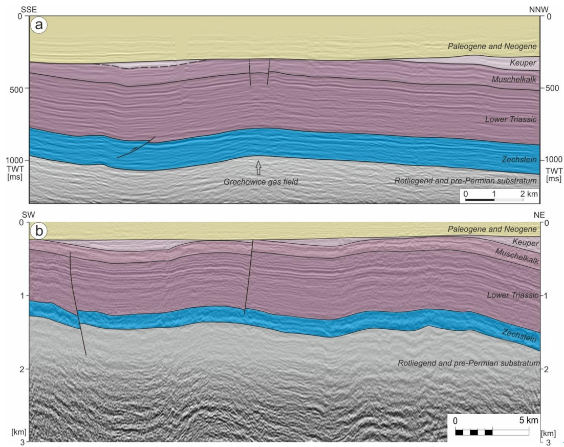
Figure 4: Two seismic profiles from the Fore-Sudetic Homocline (location in Fig. ure 2) showing very gentle folds in Triassic and Permian (Rotliegend not marked). Note steep to low-angle mainly reverse faults. The anticlines are structural traps for hydrocarbons, with gas fields known in Rotliegend strata (e.g. Grochowice gas field in Fig. ure 4a). Please note the different scales of the two profiles.
