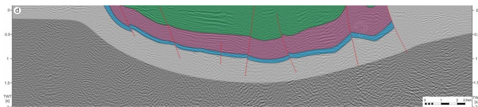
Figure- Figure 10-a-d: Interpreted seismic profiles from the North-Sudetic Synclinorium (location in Figure 6 ).
