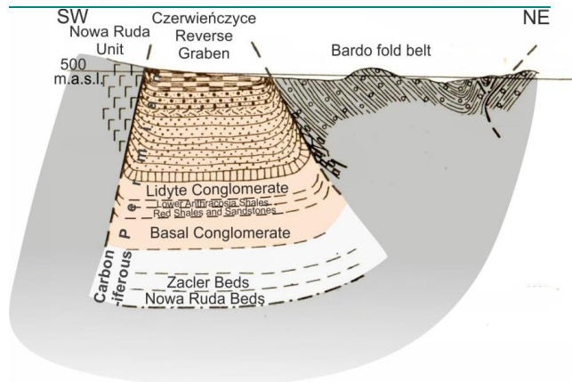
865 Figure-1516: Geological cross- section of the Czerwienicyce Reverse Graben after Oberc (1972). Location in Figs. 2 and 12.
