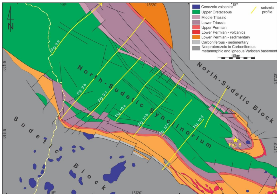
Figure 6: Geological map of the North Sudetic Synclinorium (based on Bałazińska and Bossowski, 1979; Krentz et al., 2001 and Cymerman, 2010). Locations of interpreted seismic profiles are shown. For full-length location of seismic profile of Figure 9a - see Figure 2. The map is based on Solecki (1994) and Cymerman (2010).
